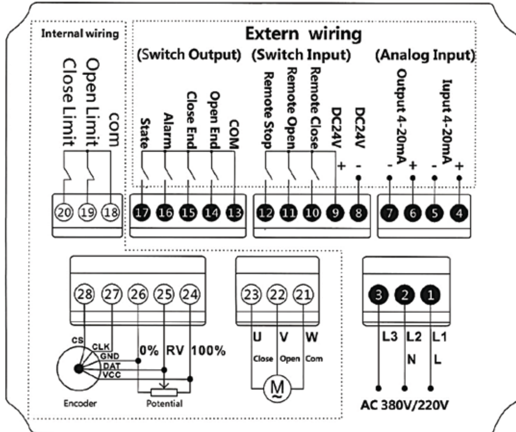
Picture 3 : Single-phase / three-phase diagram
