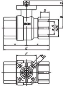
Ball valve, full bore, female/female, with DIN ISO 5211 connection for actuator, nickel-plated.
